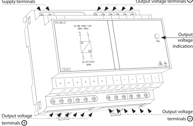
Supply terminals
